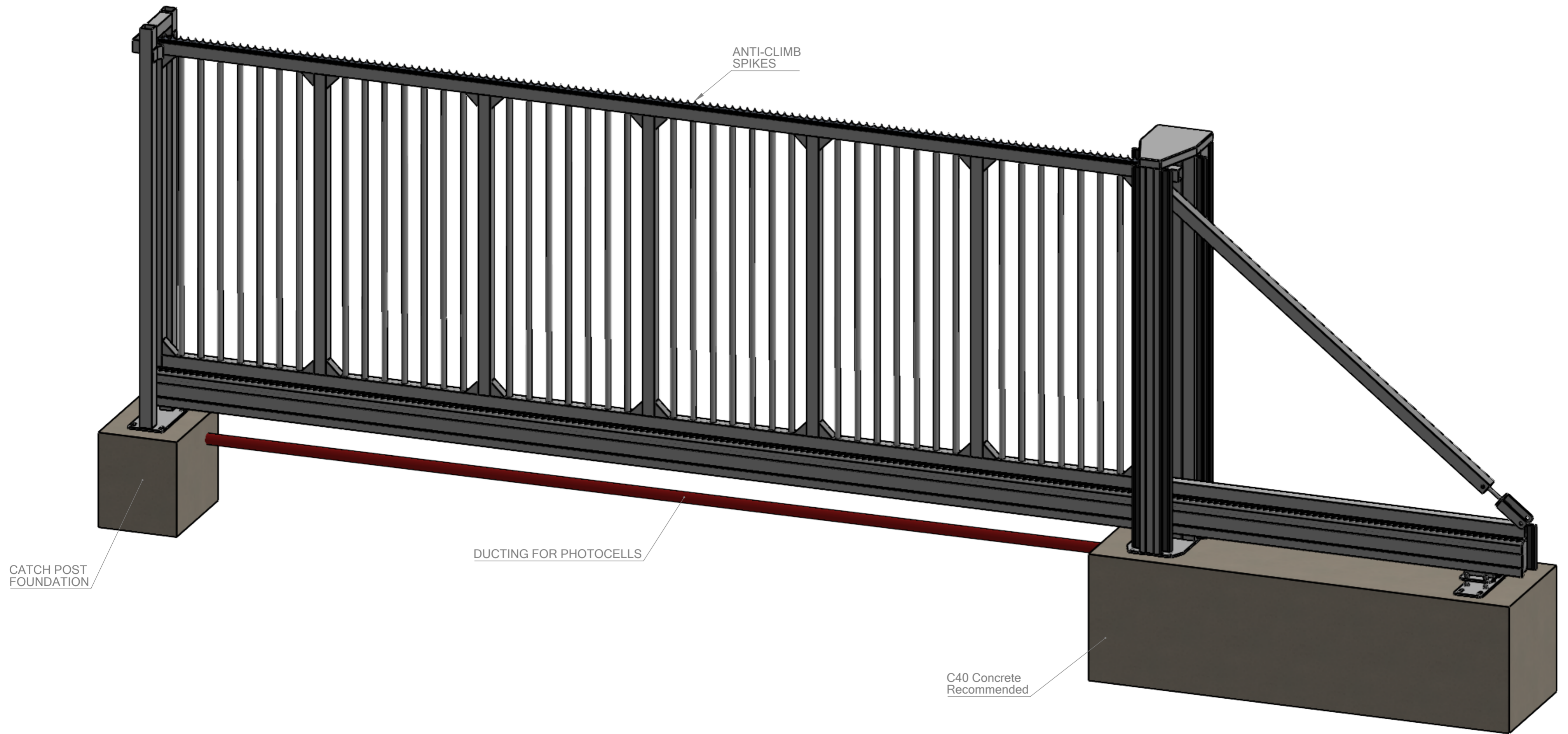
AUTO CANTILEVER SLIDING GATE 6000mm Opening x 2400mm High VERICAL BAR - Right-Handed
